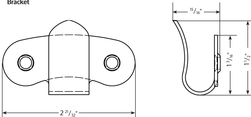
Bracket
